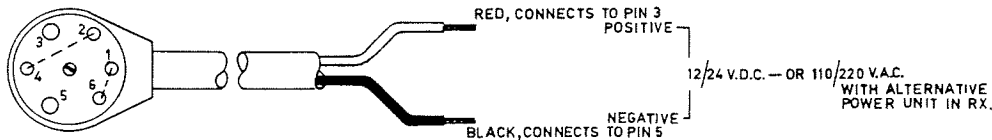
RECEIVER PLUG FEMALE HIRSCHMANN TYPE MeK 60z VIEWED FROM PIN SIDE
