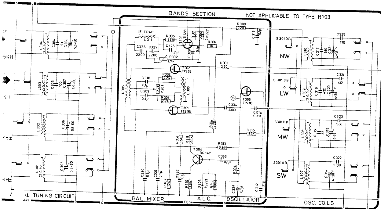
Bands section
