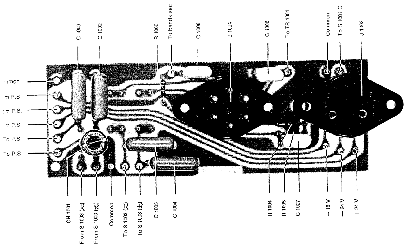
Filter section
